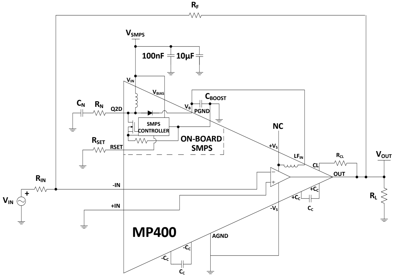
Figure 2: Typical Connection
